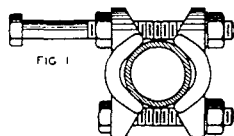
Clamping Bolt is Extension Arm
